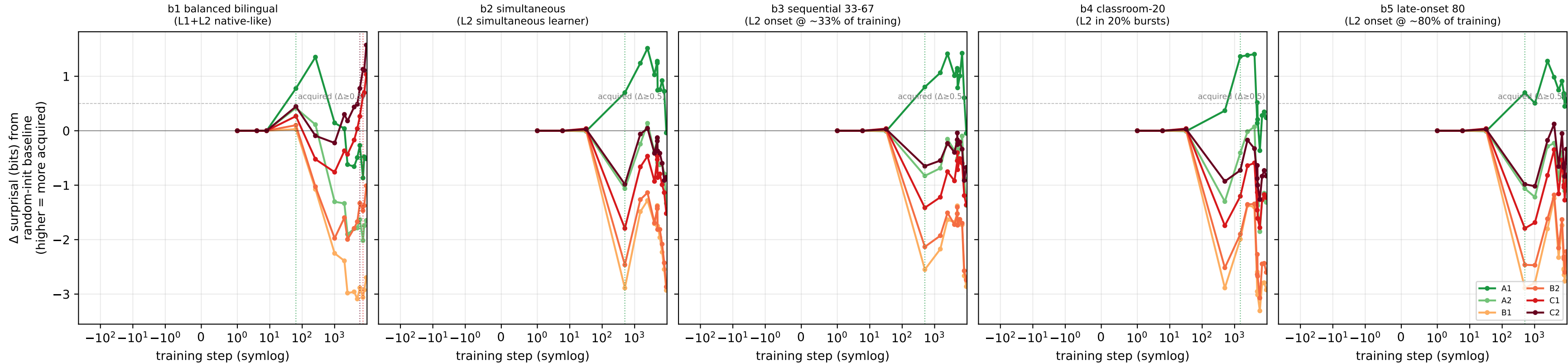
Per-curriculum CEFR-aligned learner trajectory (HumanScale) — \Delta(\text{surprisal}) from random-init baseline. Vertical markers = first checkpoint where \Delta \geq 0.5 bits. Curricula b2-b5 progress through CEFR stages in canonical order; the marker step IS the simulator checkpoint for that CEFR level.
